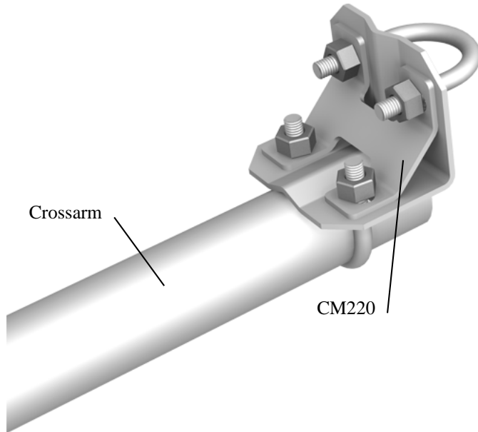
FIGURE 7-2. The CM220 mounted to a crossarm
